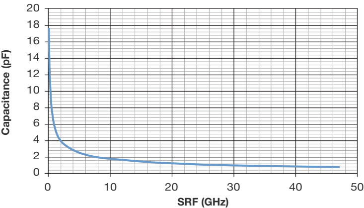
Accu-P® 0805 Typical SRF vs Capacitance
